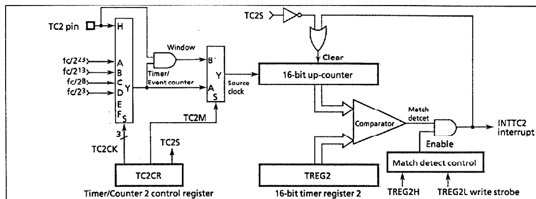
Figure 2-19. Timer/counter 2 (TC2)
