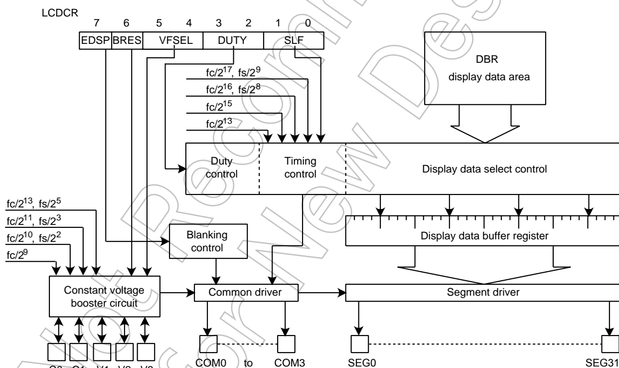
Figure 13-1 LCD Driver
