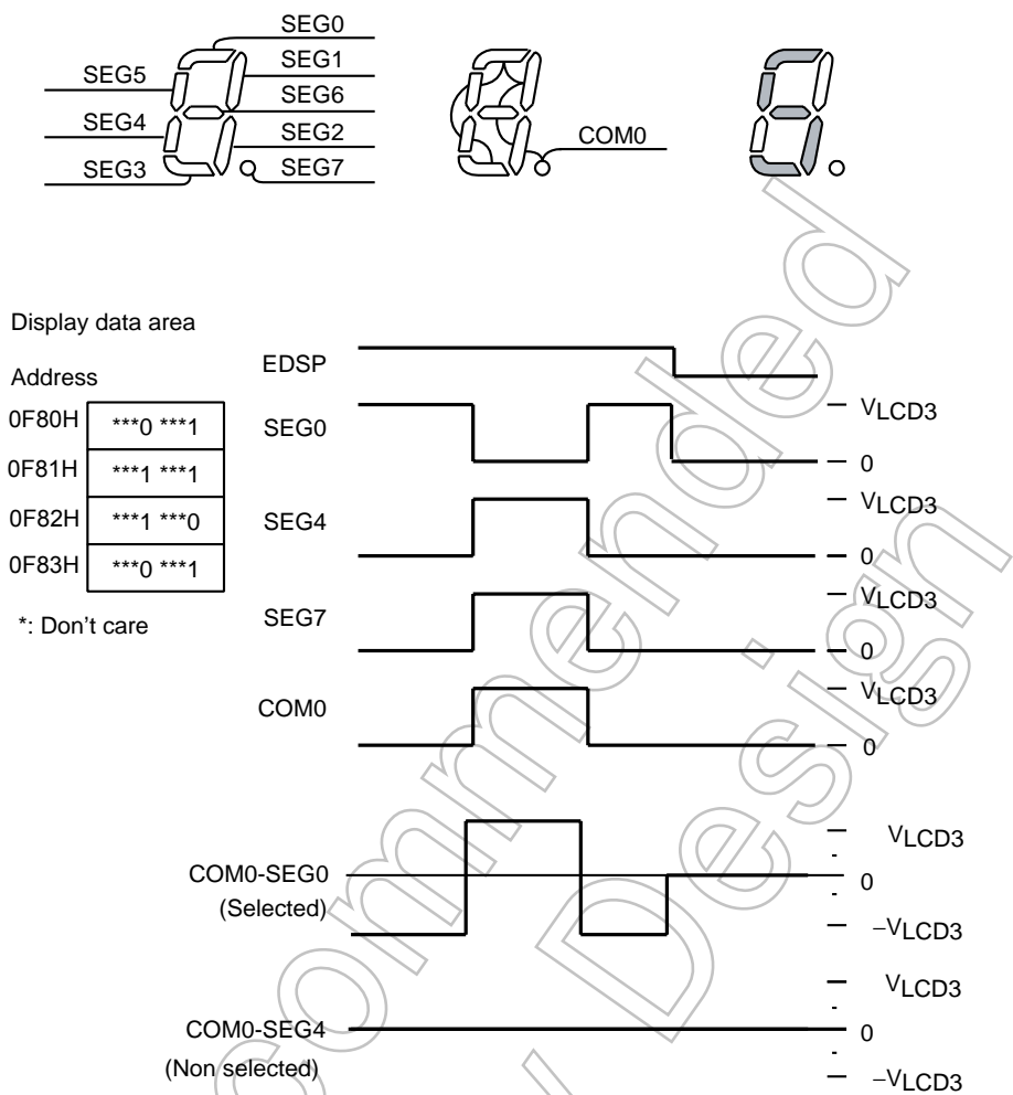
Figure 13-11 Static Drive
