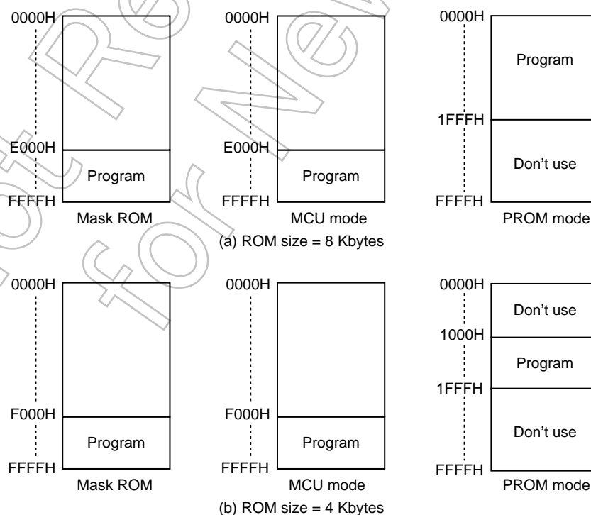
Figure 14-1 Program Memory Area
