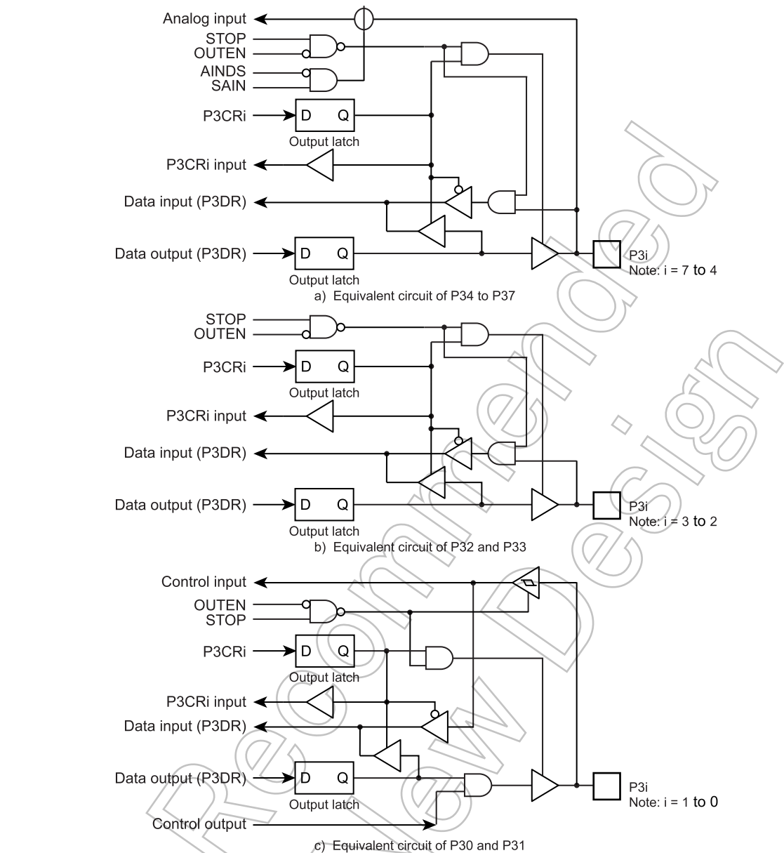
Figure 5-5 Port P3
