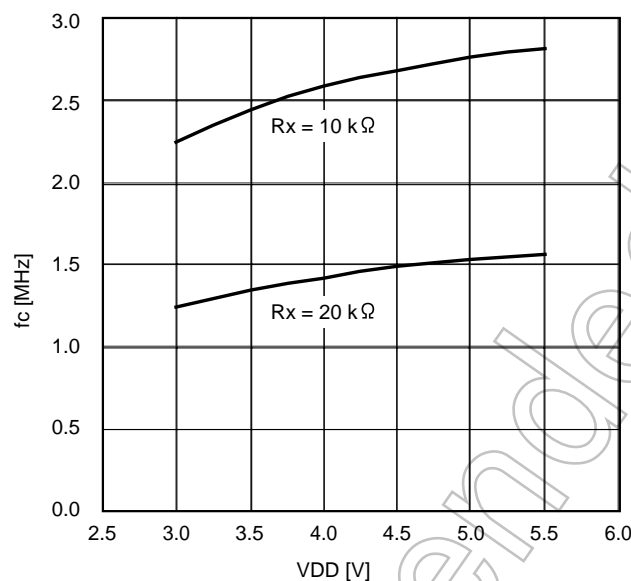
Figure 12-2 Oscillation Frequency ( f_c ) vs VDD ( C = 33 pF, T_a = 25^\circ\text{C} )
