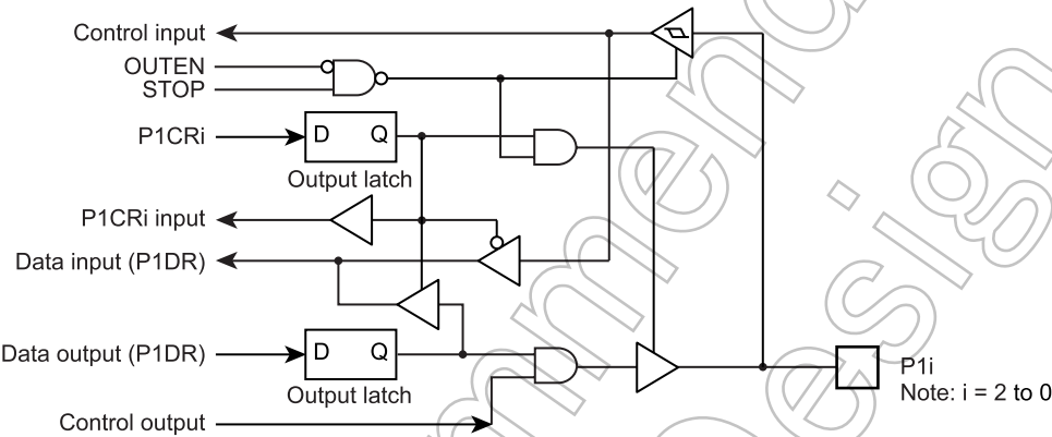
Figure 5-3 Port P1
