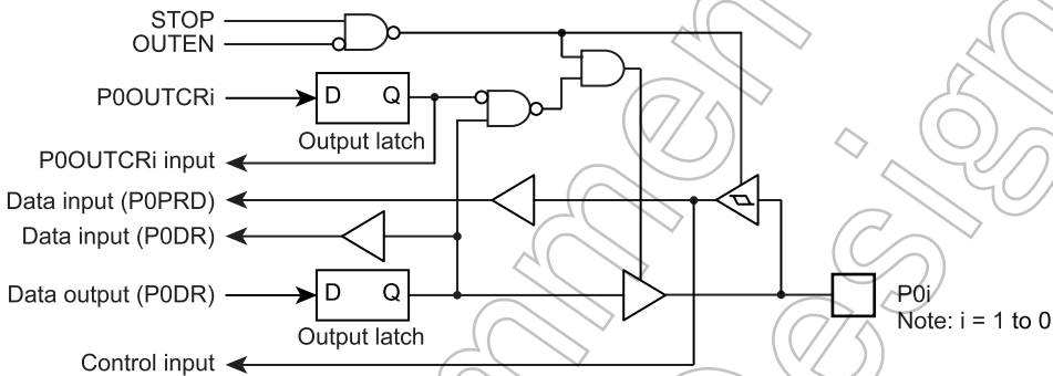
Figure 5-2 Port P0
