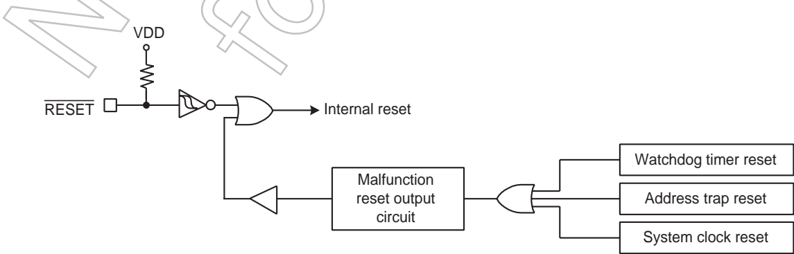
Figure 2-14 Reset Circuit
