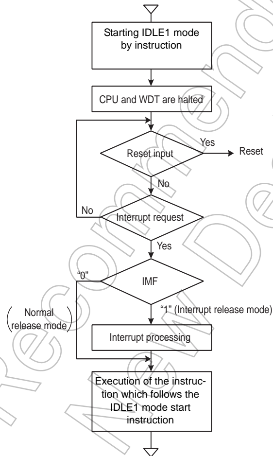
Figure 2-10 IDLE1 Mode
