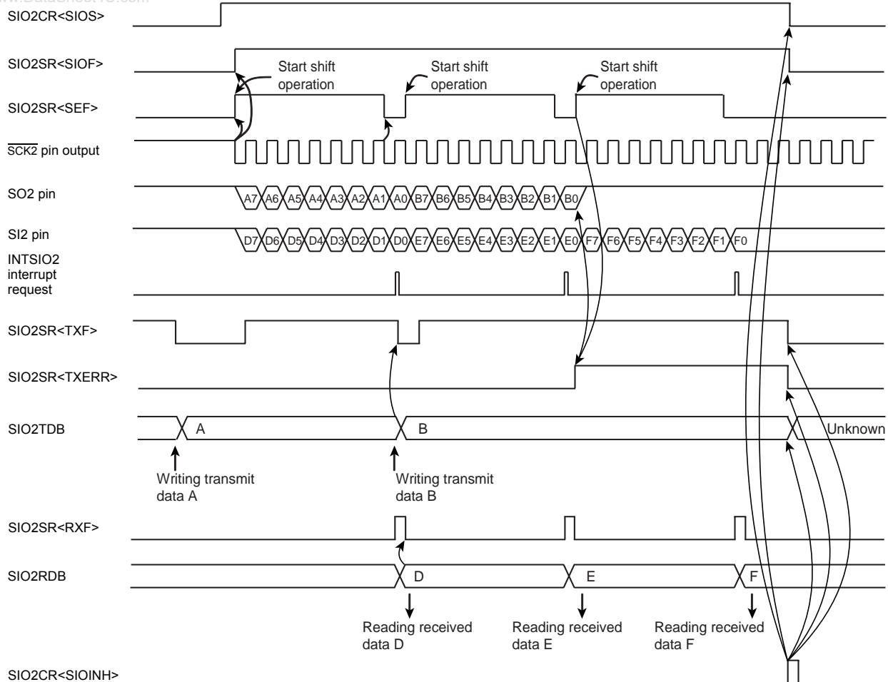
Figure 15-15 Example of Transmit/Receive (Transmit) Error Processing
