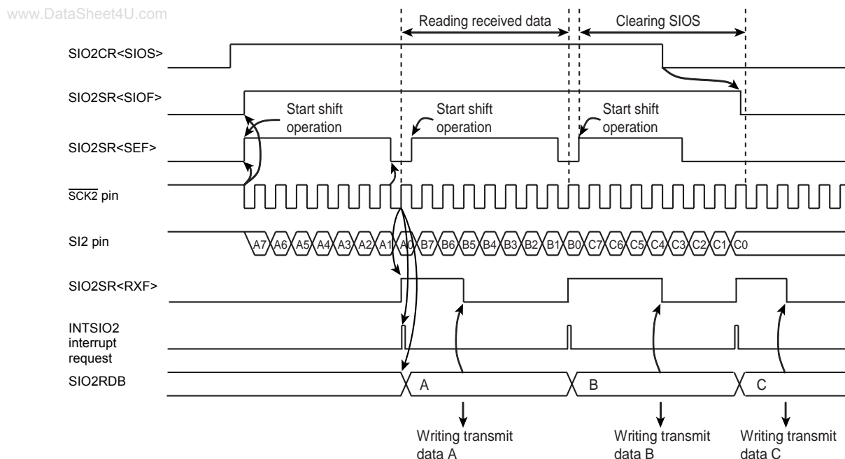
Figure 15-11 Example of External Clock and MSB Receive Mode
