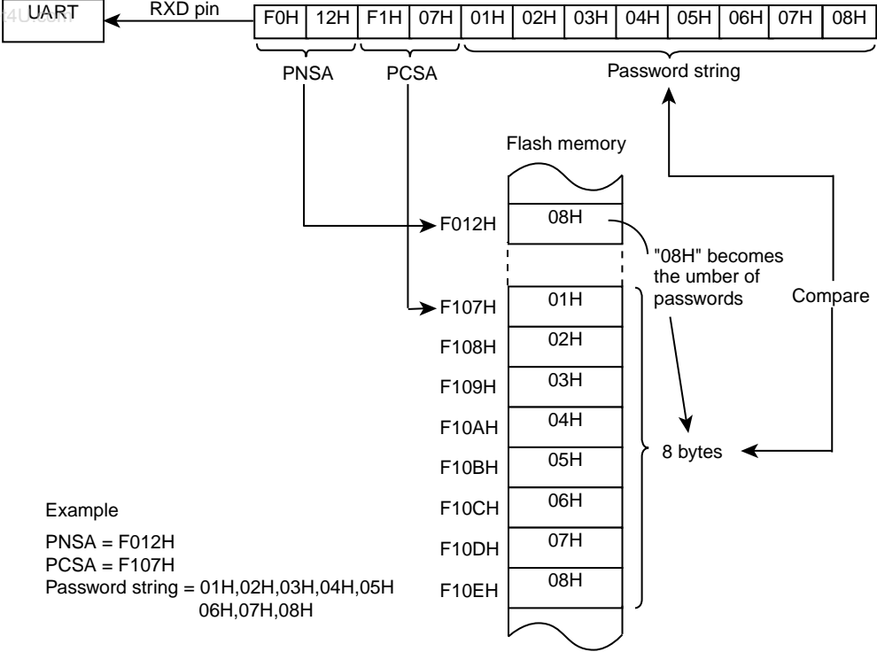
Figure 20-5 Password Comparison
