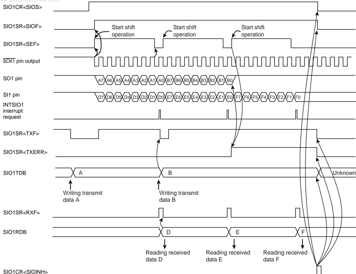
Figure 14-15 Example of Transmit/Receive (Transmit) Error Processing
