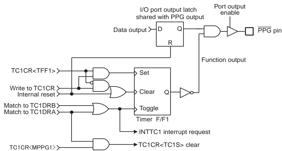
Figure 8-7 PPG Output
