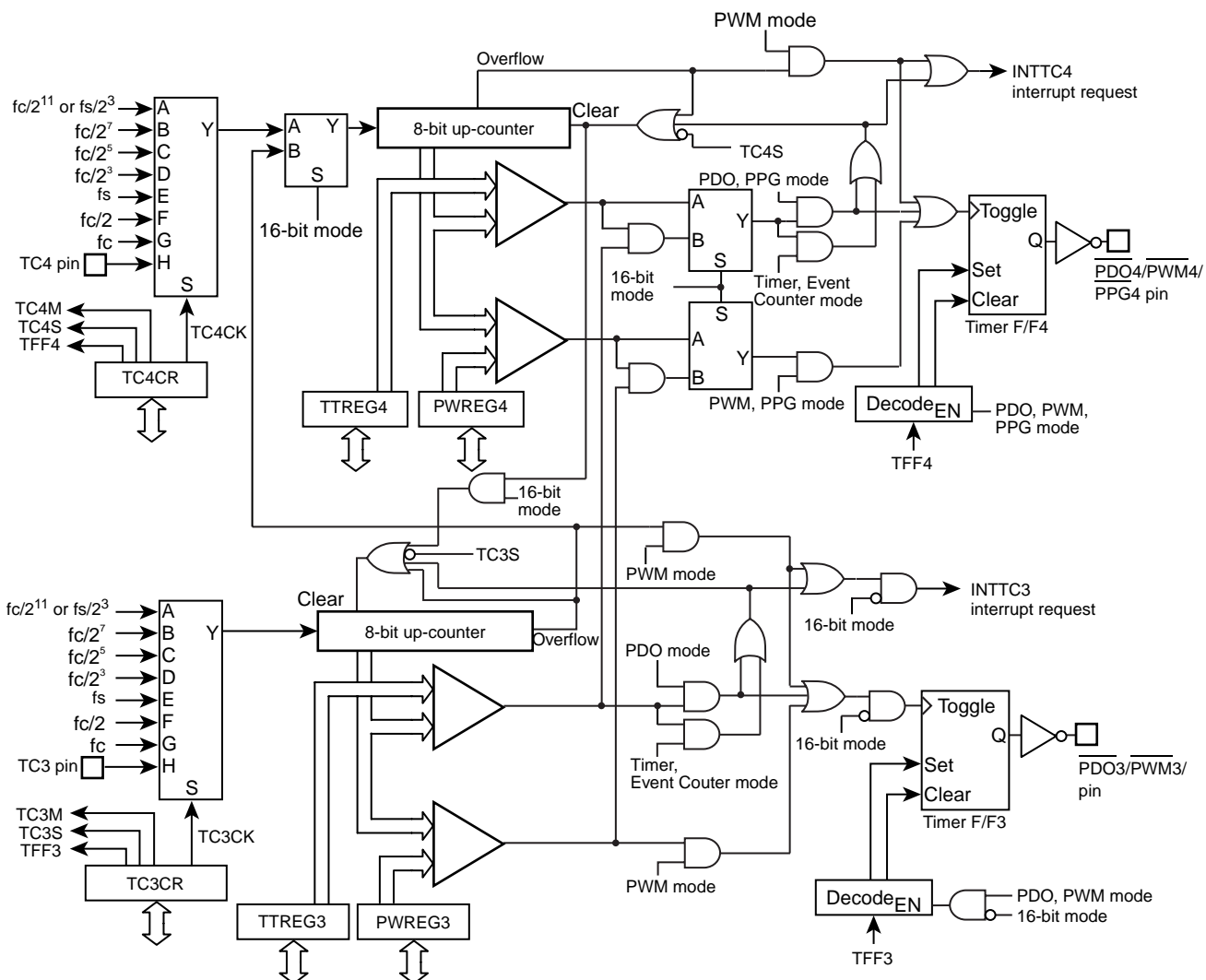
Figure 10-1 8-Bit TimerCounter 3, 4
