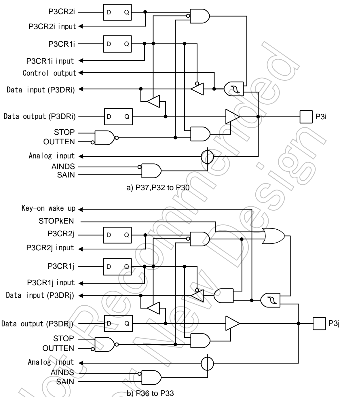
Figure 5-5 Port 3
