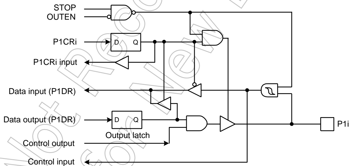
Figure 5-3 Port 1
