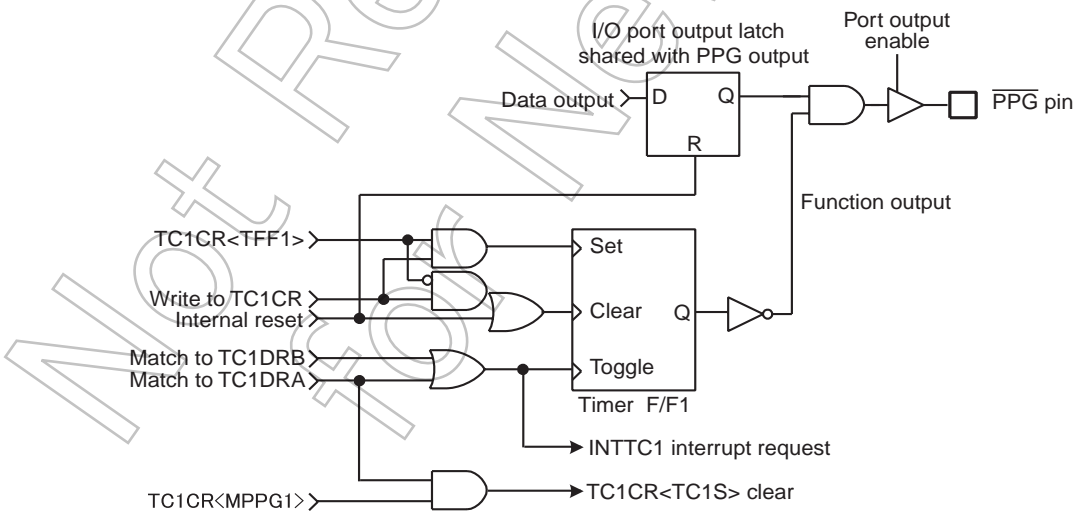
Figure 10-7 \overline{\text{PPG}} Output
