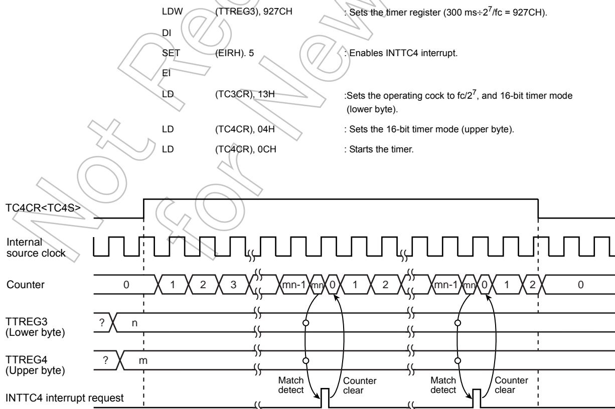
Figure 11-6 16-Bit Timer Mode Timing Chart (TC3 and TC4)
