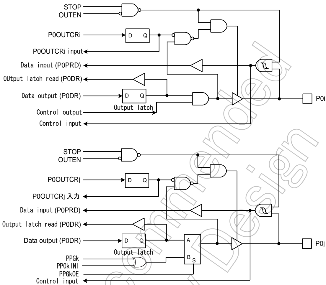
Figure 5-2 Port 0
