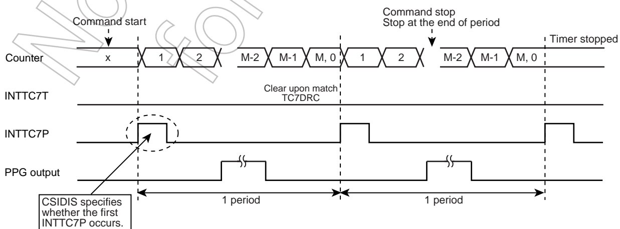
Figure 9-21 Period Interrupt
