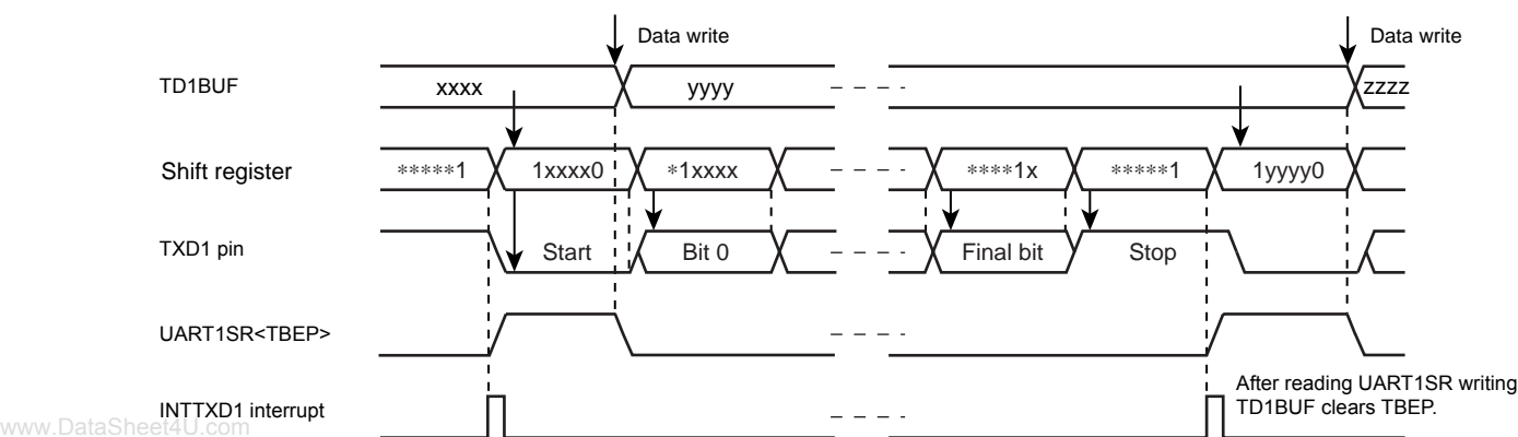
Figure 12-9 Generation of Transmit Data Buffer Empty
