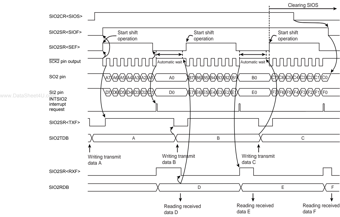
Figure 15-13 Example of Internal Clock and MSB Transmit/Receive Mode
