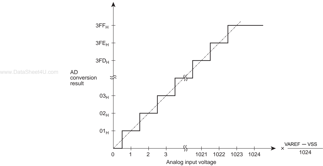
Figure 17-4 Analog Input Voltage and AD Conversion Result (Typ.)
