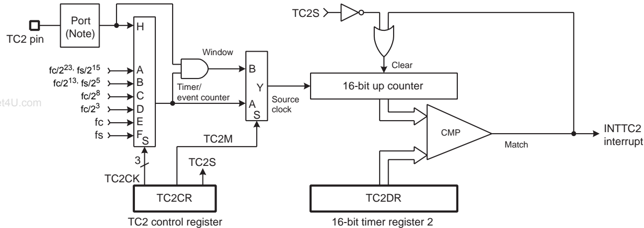
Figure 9-1 Timer/Counter2 (TC2)
