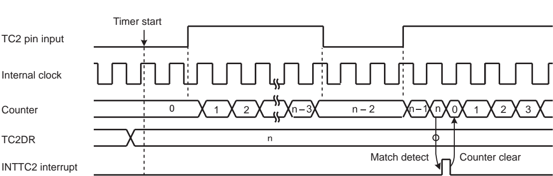
Figure 9-4 Window Mode Timing Chart
