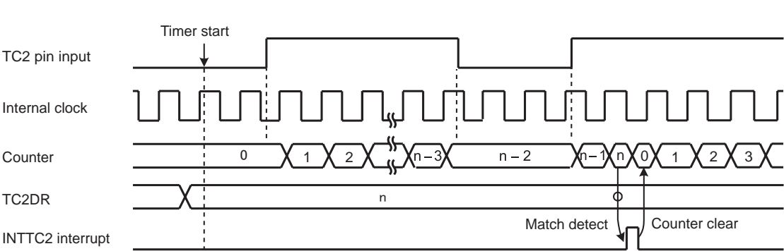
Figure 9-4 Window Mode Timing Chart
