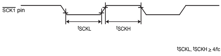
Figure 14-3 External Clock
