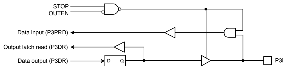
Figure 5-5 Port 3
