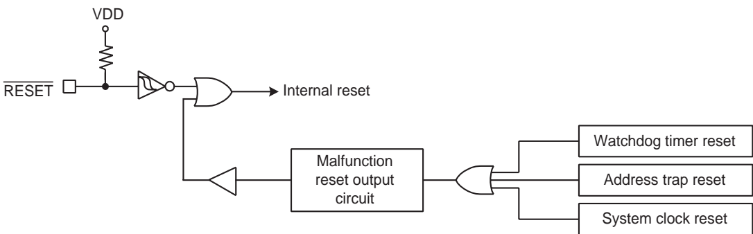
Figure 2-15 Reset Circuit
