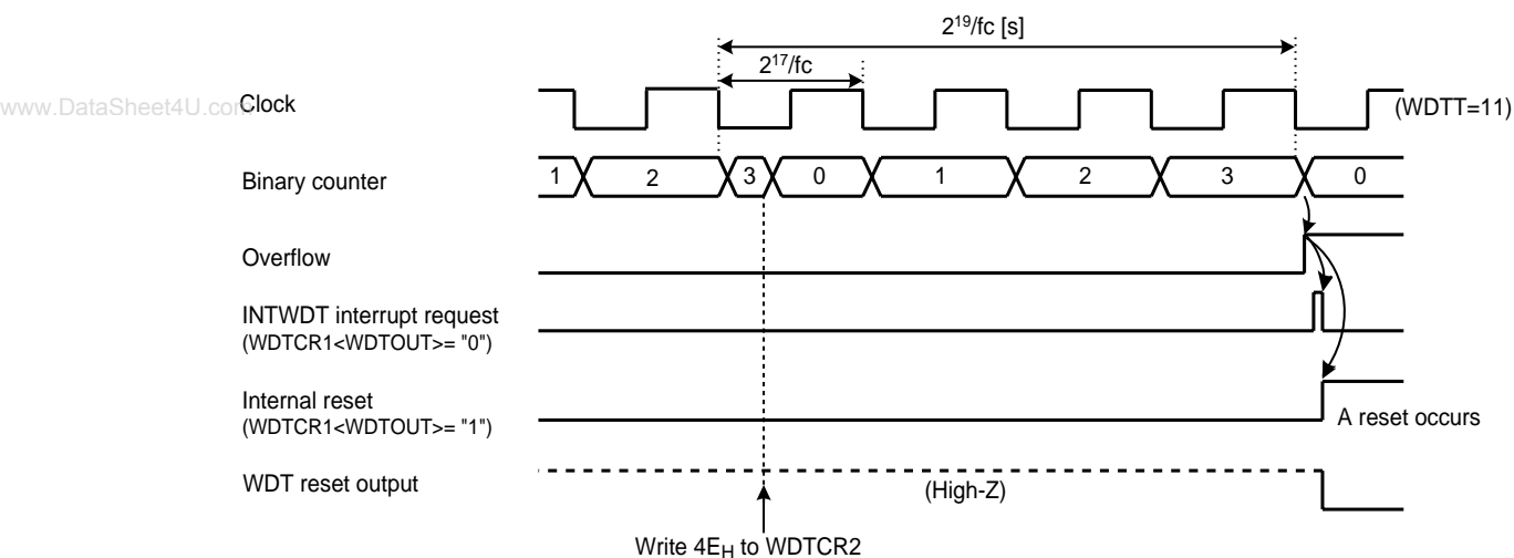
Figure 6-2 Watchdog Timer Interrupt/Reset
