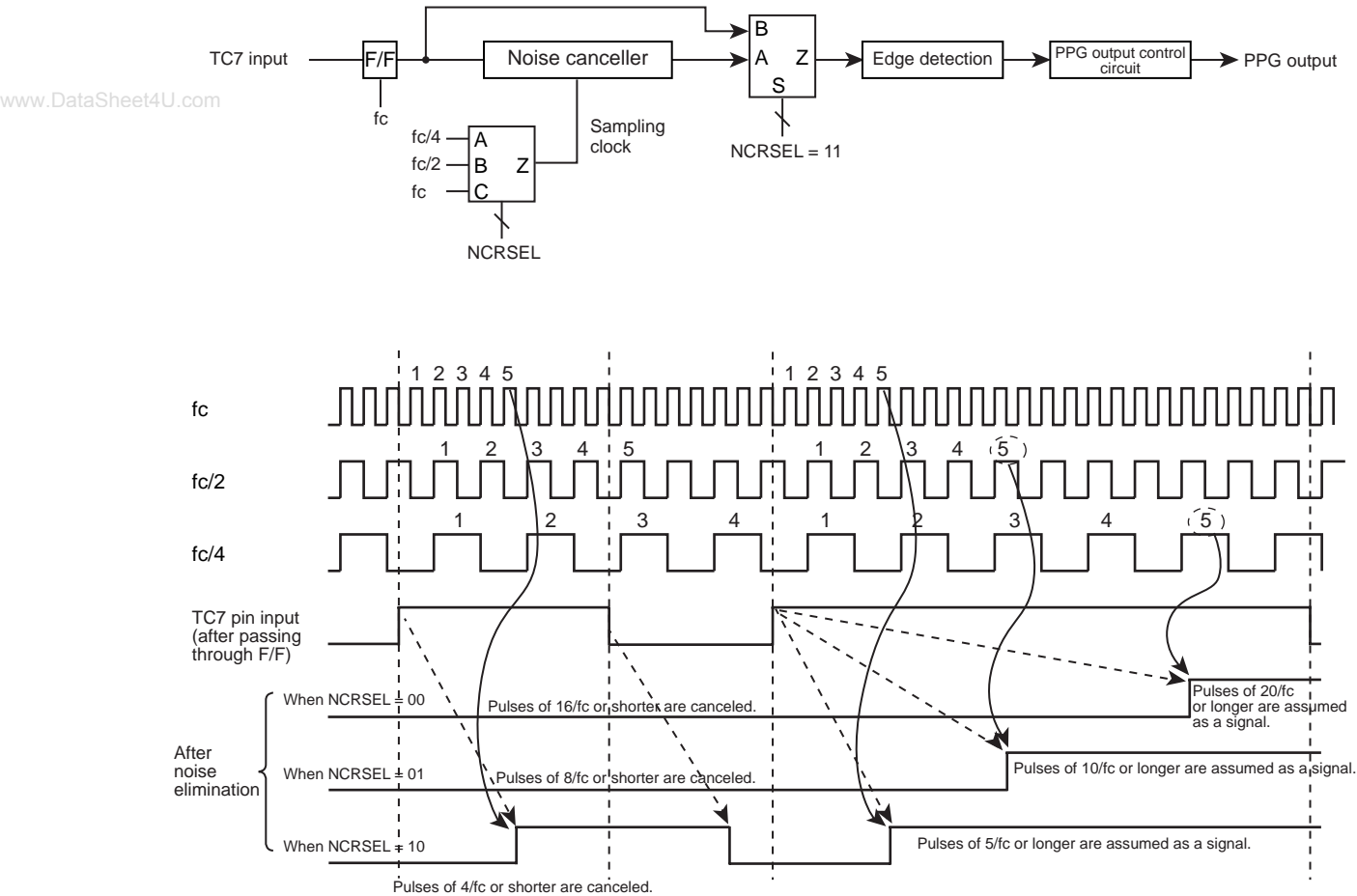
Figure 8-19 Noise Canceller Operation
