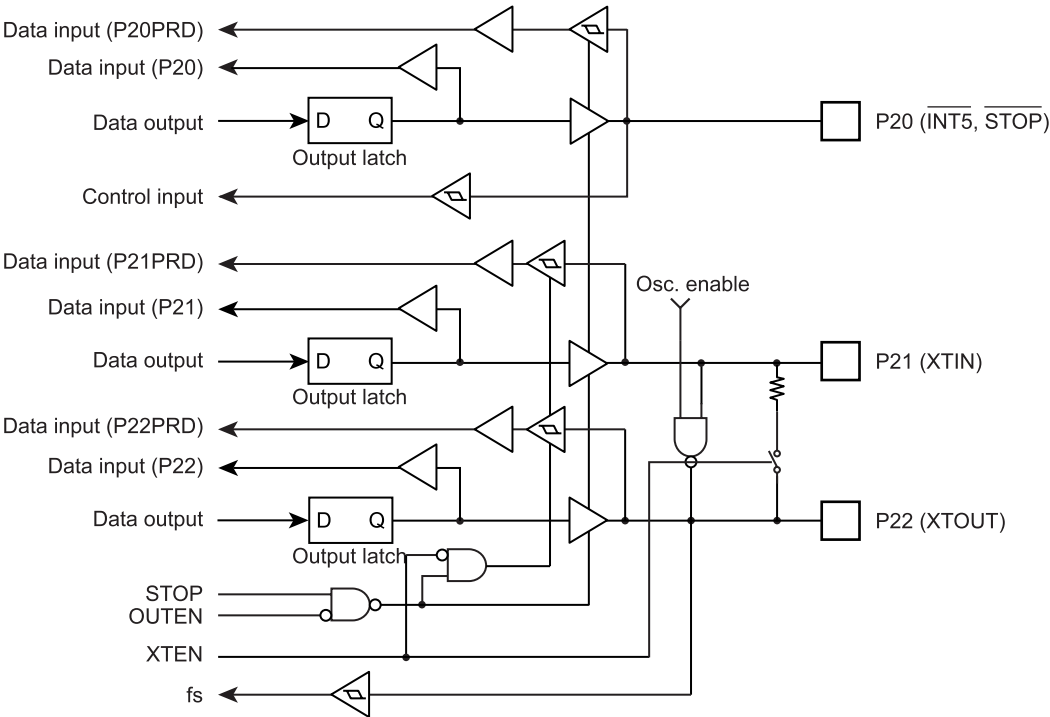
Figure 5-4 Port P2
