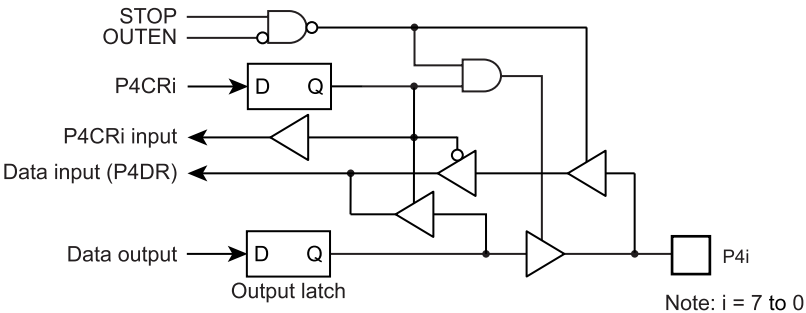
Figure 5-6 Port P4
