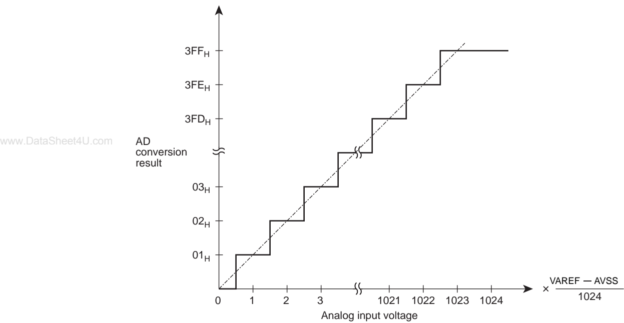
Figure 12-4 Analog Input Voltage and AD Conversion Result (Typ.)
