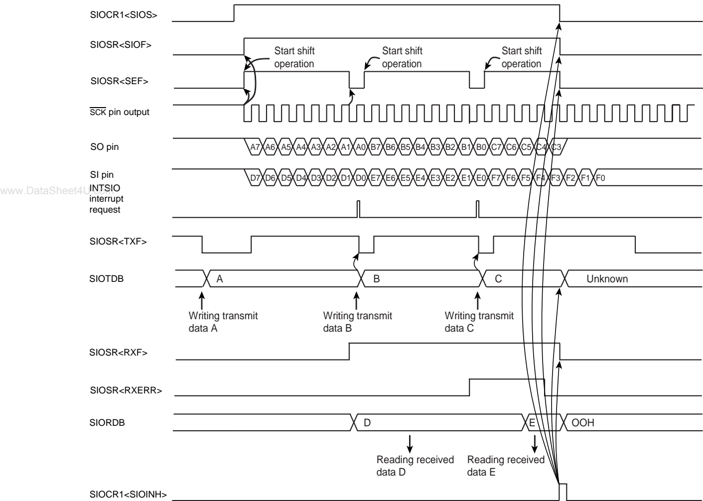
Figure 10-16 Example of Transmit/Receive (Receive) Error Processing
