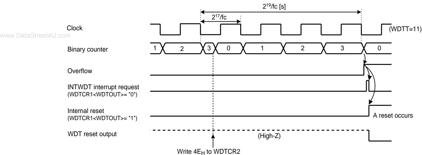
Figure 7-2 Watchdog Timer Interrupt/Reset
