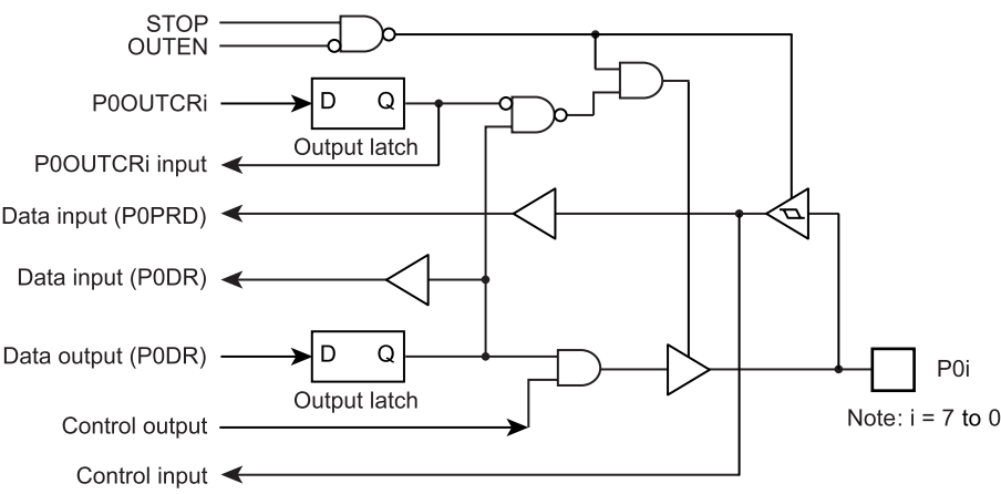
Figure 5-2 P0 Port
