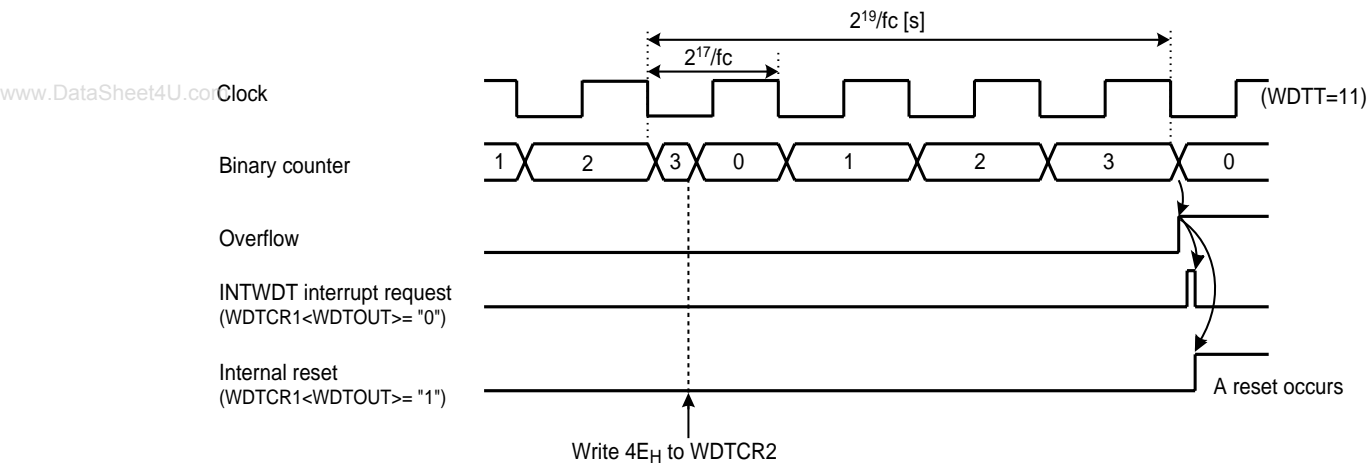
Figure 7-2 Watchdog Timer Interrupt
