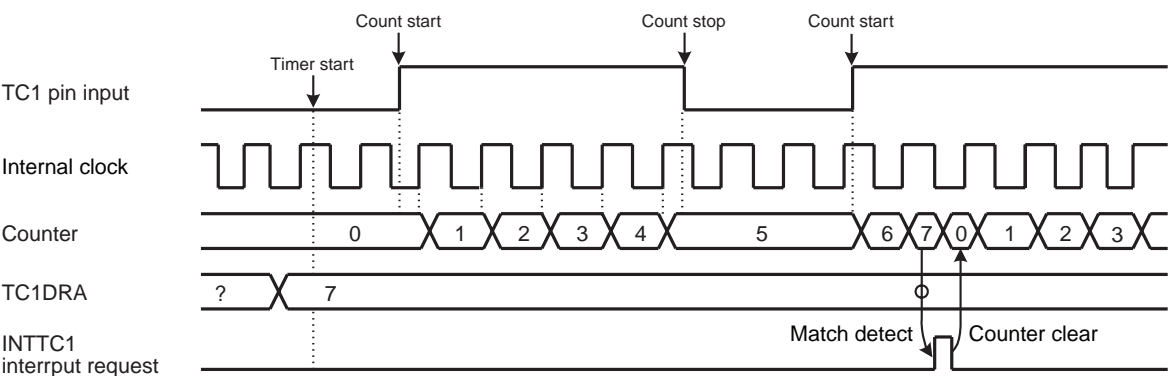
(a) Positive logic (TC1S = 10)
