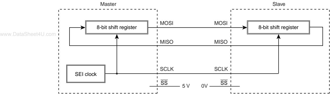
Figure 11-4 Master and Slave Connection in SEI
