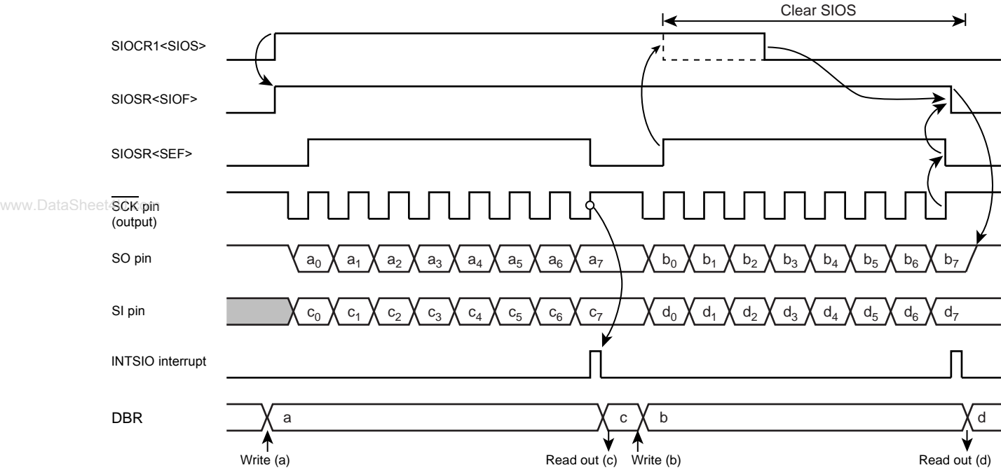
Figure 10-11 Transfer / Receive Mode (Example: 8bit, 1word transfer, Internal clock)
