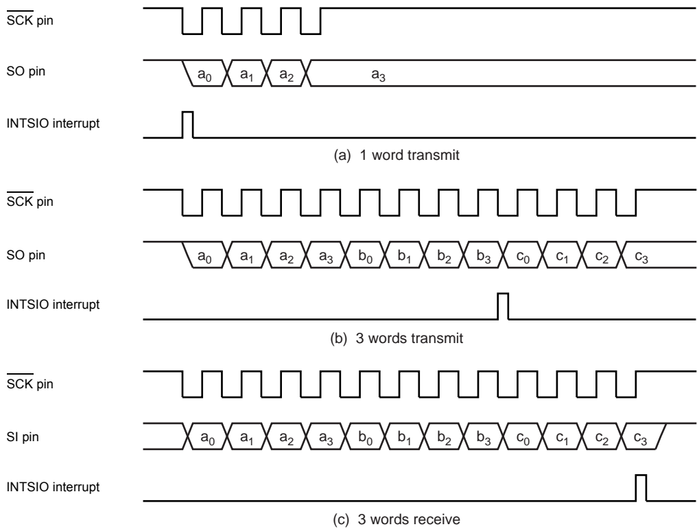
Figure 10-6 Number of words to transfer (Example: 1word = 4bit)
