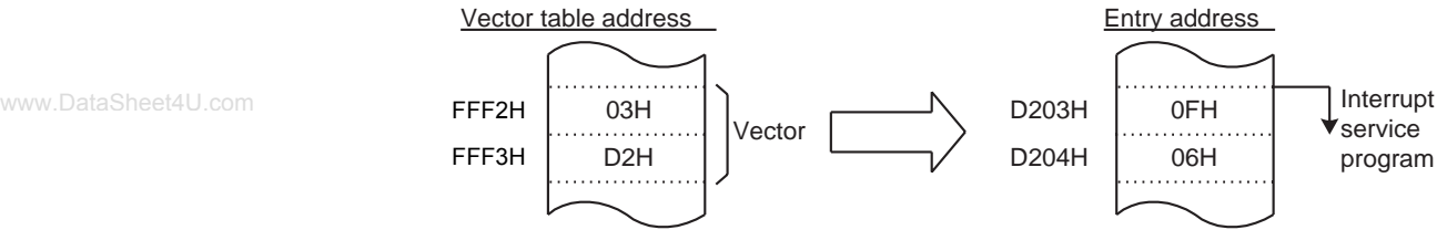
Figure 3-2 Vector table address,Entry address
