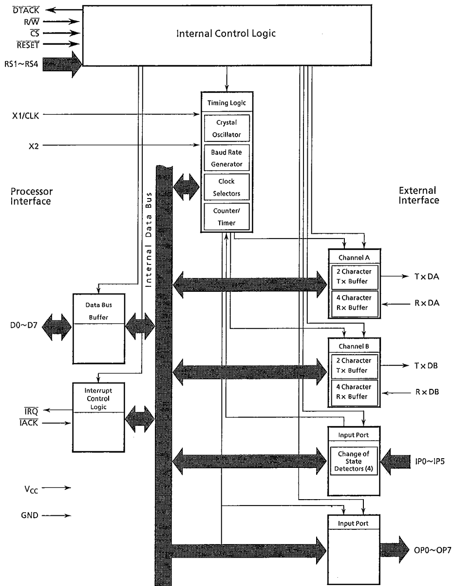
Figure 1.1 Block Diagram
