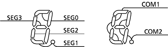
Figure 3.12 Example of COM and SEG connection.
