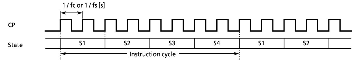
Figure 2-4. Instruction Cycle
