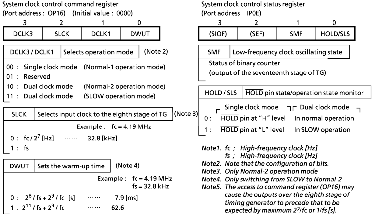
Figure 2-2. System Clock Control Command Register
