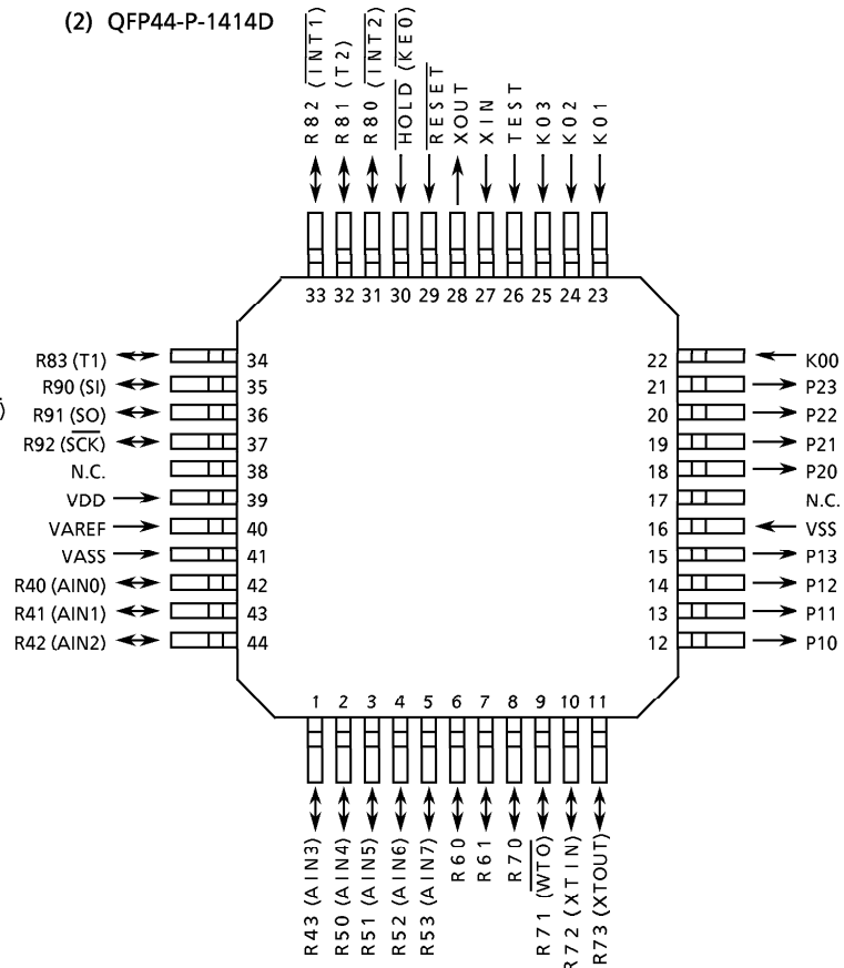
(2) QFP44-P-1414D
