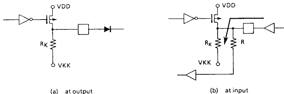
Figure 2-14. Input/Output interface
