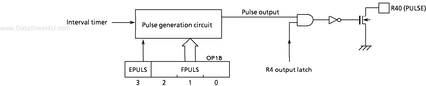
Figure 3-9. Pulse output circuit
