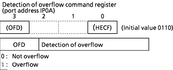
Figure 3-8. Detection of overflow command register
