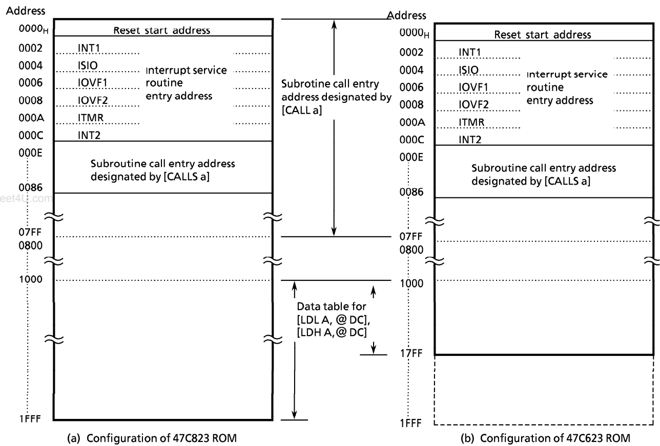
Figure 2-2. Program Memory Map
