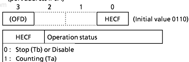
Figure 3-6. HEC operation status register
