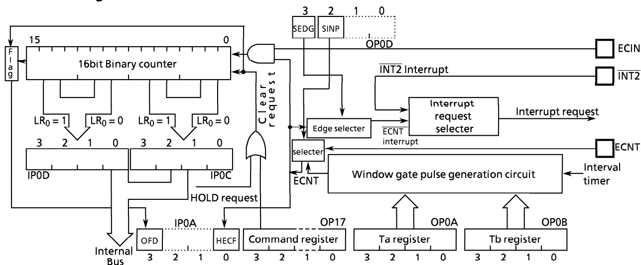
Figure 3-3. Configuration of High Speed Event/Counter
