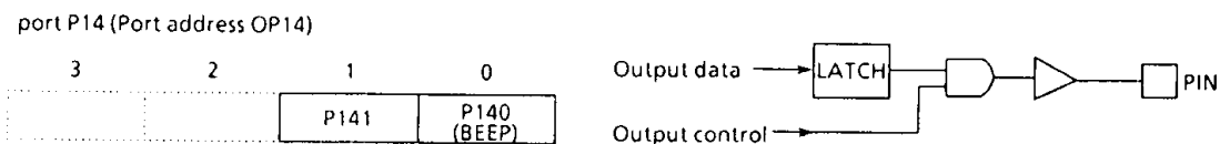
Figure 3-3. Port P14
