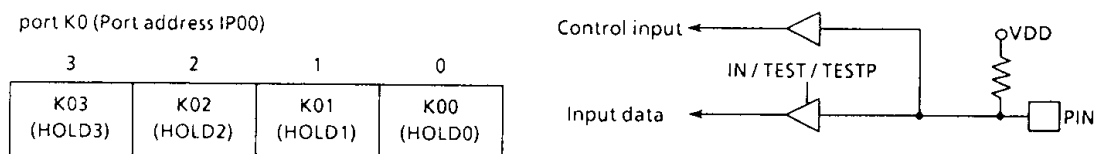
Figure 3-1. Port K0
