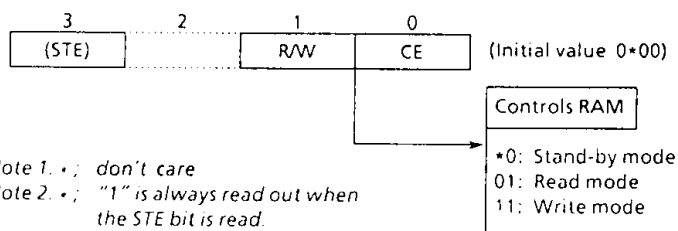
Figure 2-4. RAM Command Register
