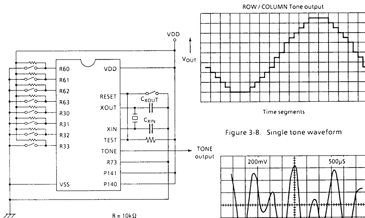
Figure 3-7. Tone test circuit
