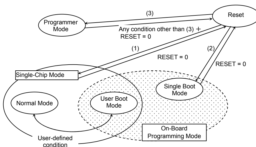
Figure 17.2.1 Mode Transitions
