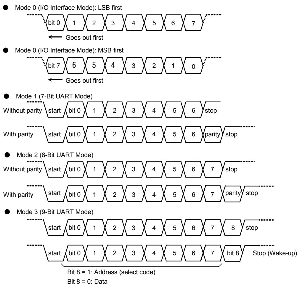
Figure 12.1.1 Data Formats
