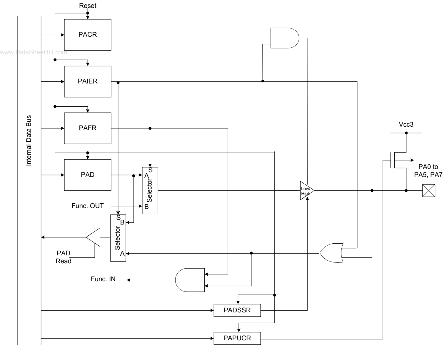
Figure 8.10.1 Port A (PA0 to PA5, PA7)
