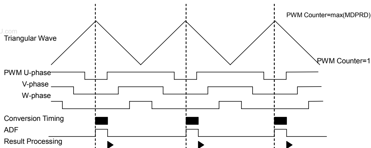
Figure 13.6.1 AD Converter Example of Use 1 Timing
