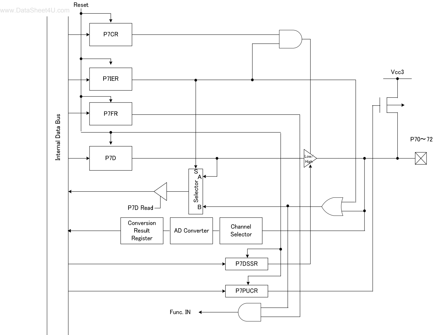
Figure 8.7.1 Port 7 (P70 to P72)
