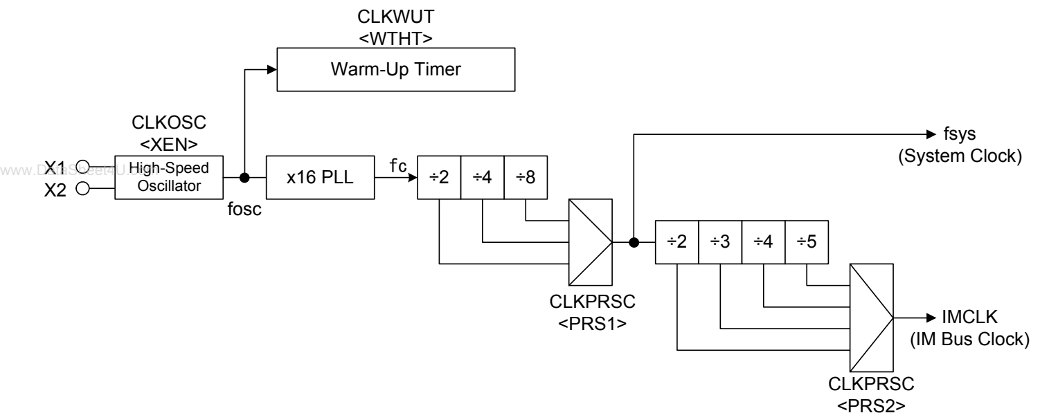
Figure 5.2.1 Clock Source Block Diagram
