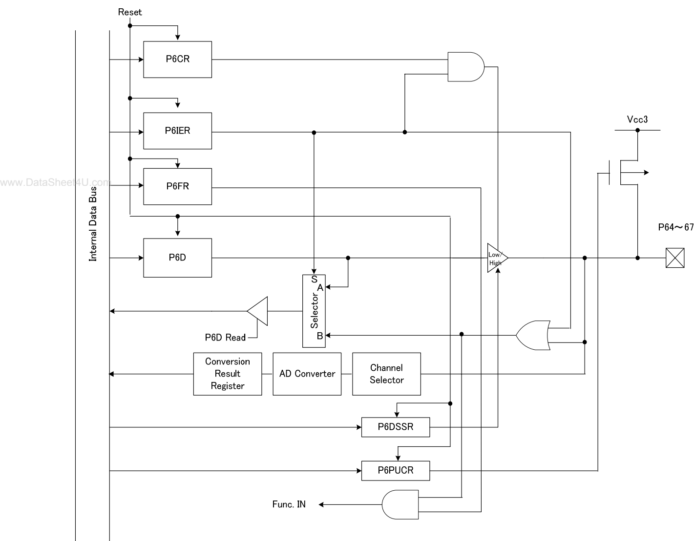
Figure 8.6.2 Port 6 (P64 to P67)
