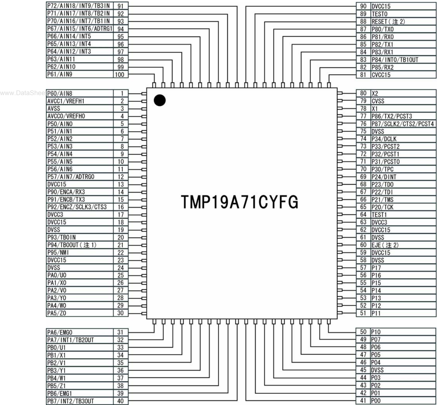
Figure 2.2 TMP19A71CYFG Pin Assignments (100-pin QFP)
