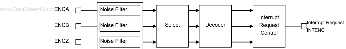
Figure 15.1.1 Block Diagram of the Encoder Input Circuit
