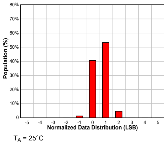
Figure 8-13. Data Distribution With 3-ms Conversion Time and Averaging On in 16-Bit Format
