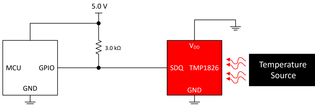
Figure 10-1. Bus Powered Application
