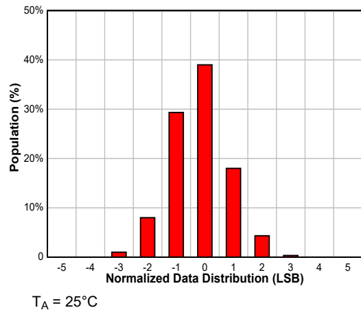
Figure 8-14. Data Distribution With 5.5-ms Conversion Time and Averaging Off in 16-Bit Format
