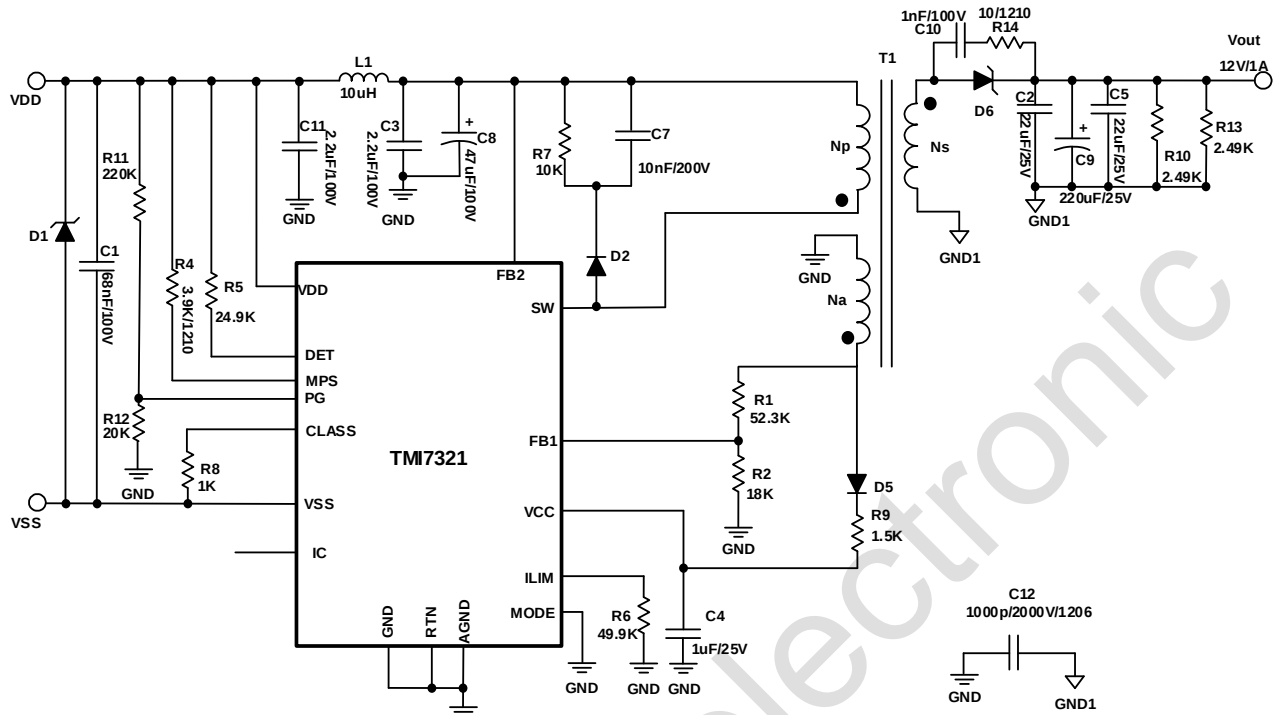
TMI7321 Flyback Typical Application Circuit
