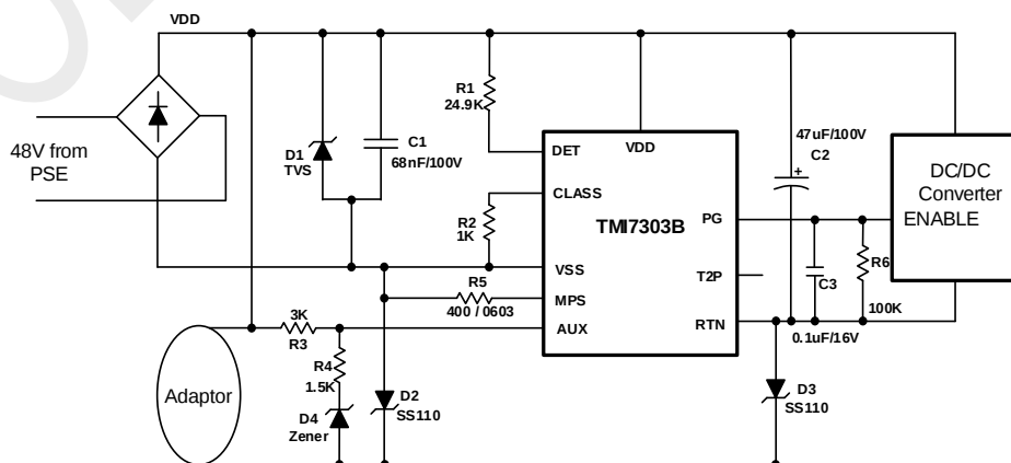
Figure 1. TMI7303B Typical Application Circuit
