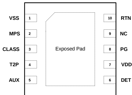
DFN3x3-10
