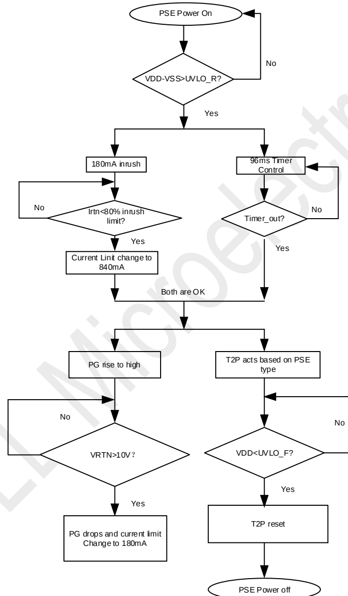
Figure 4: Startup Sequence
