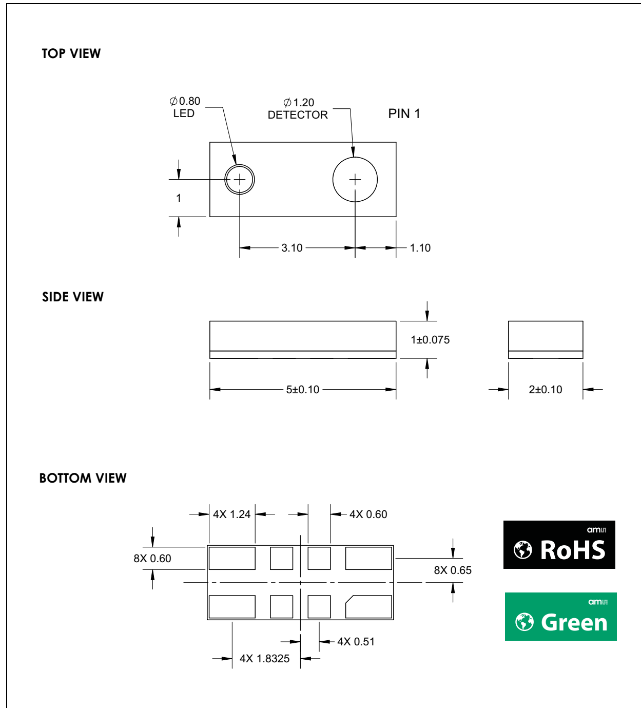
Figure 99: TMG4903 Module Dimensions
