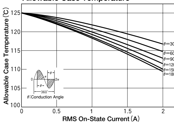
RMS On-State vs Allowable Case Temperature
