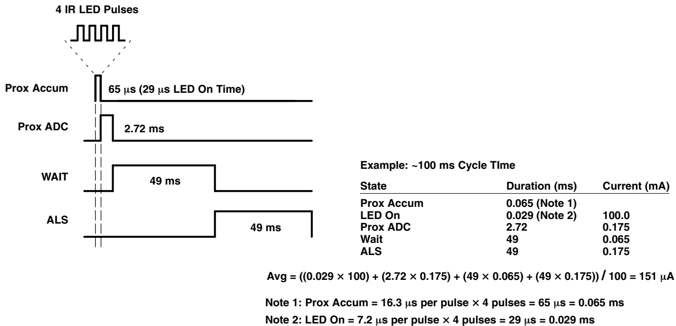
Figure 11. Power Consumption Calculations
