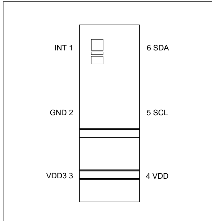
Figure 3: Pin Diagram
