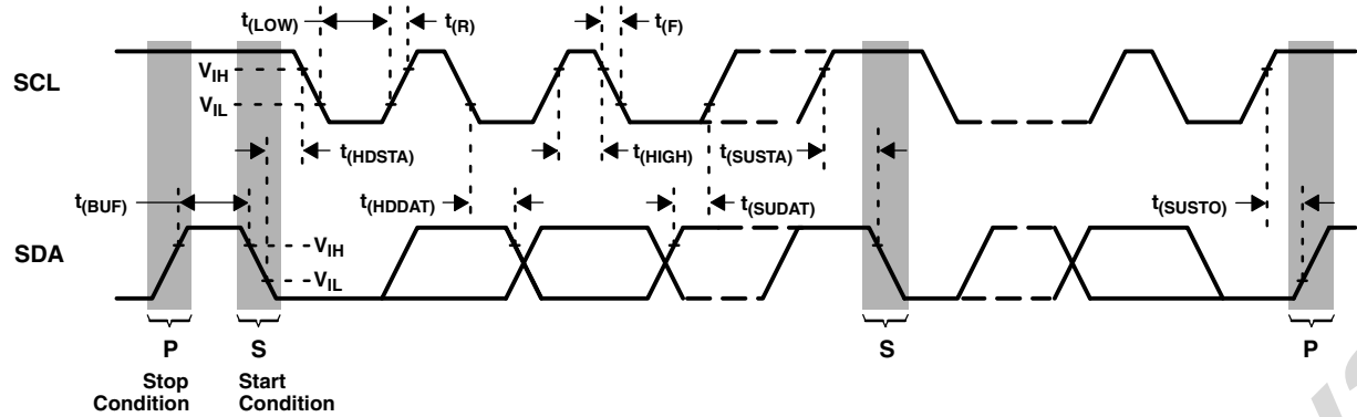
Figure 1. Timing Diagrams
