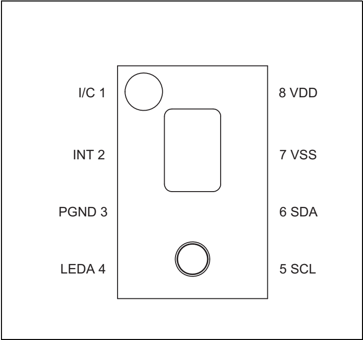
Figure 3: TMD2620 Pinout (Top View)
