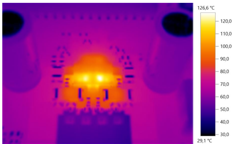
Figure 28.1 Thermal photo showing 3.5A RMS operation with SpreadCycle on TMC5161-EVAL
