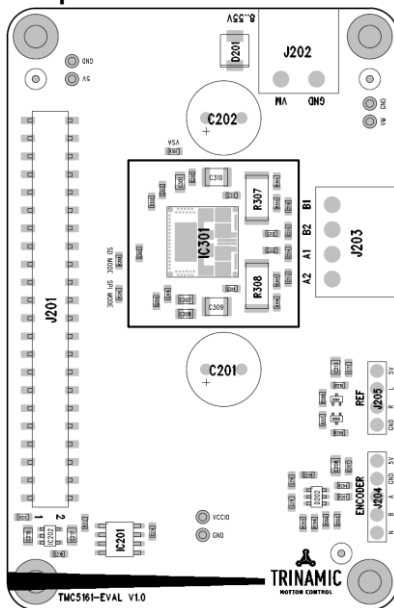
Figure 29.1 Layout example
