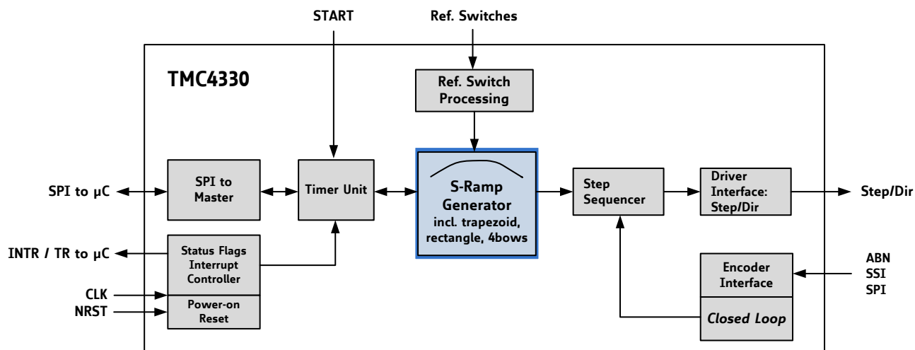
Figure 2: Block Diagram
