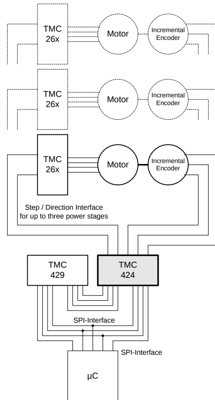
TMC424 as Step / Direction converter and Incremental Encoder Interface
