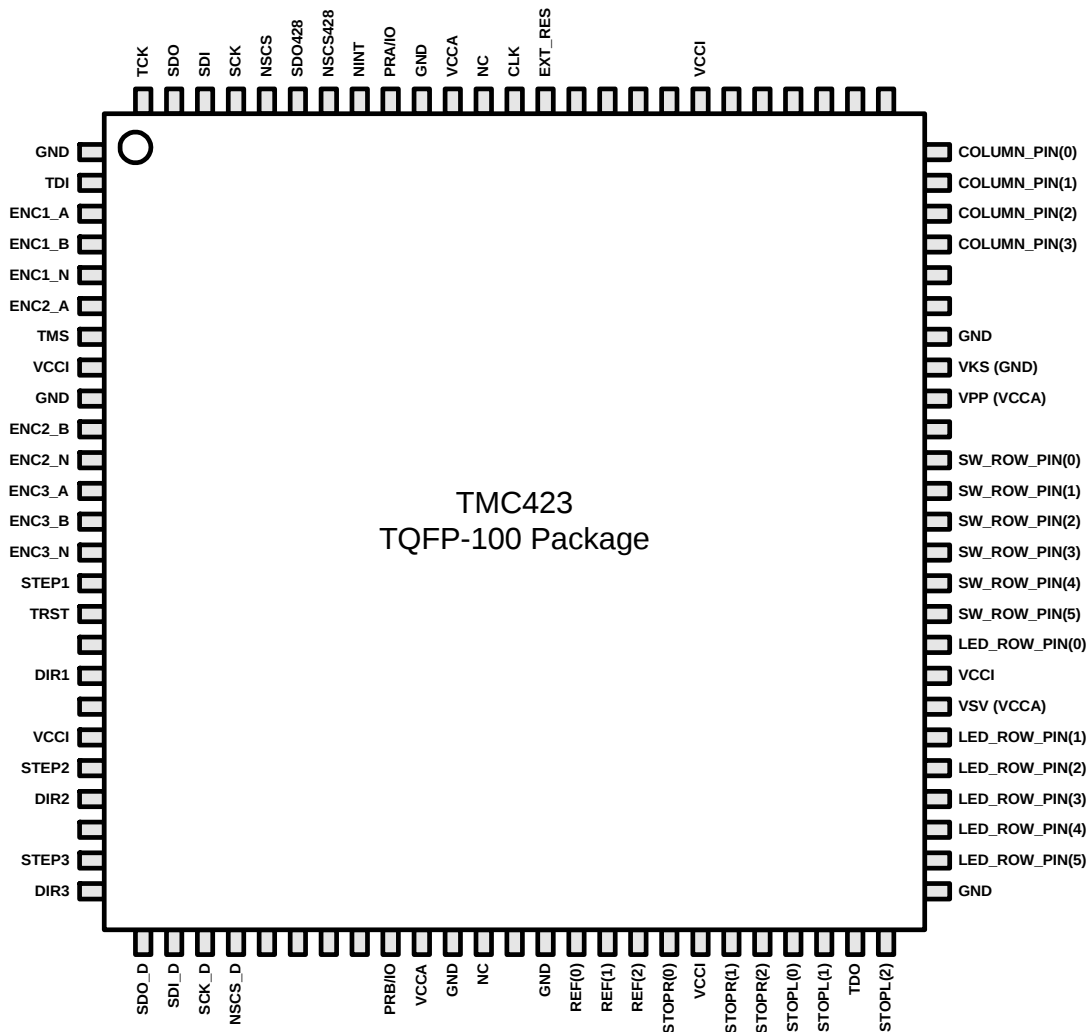
Figure 1: Pinout TMC423
