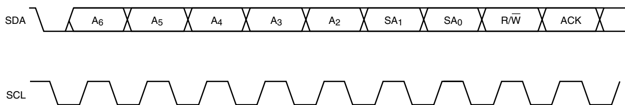
Figure 28. Serial Interface – Chip Address
