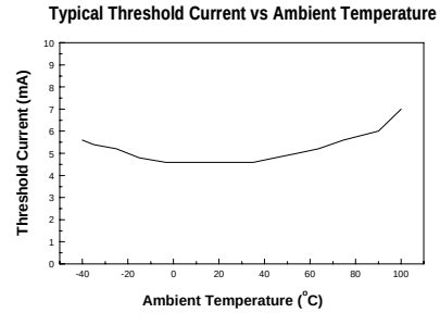
Fig. 4 Temperature Dependence of Threshold Current
