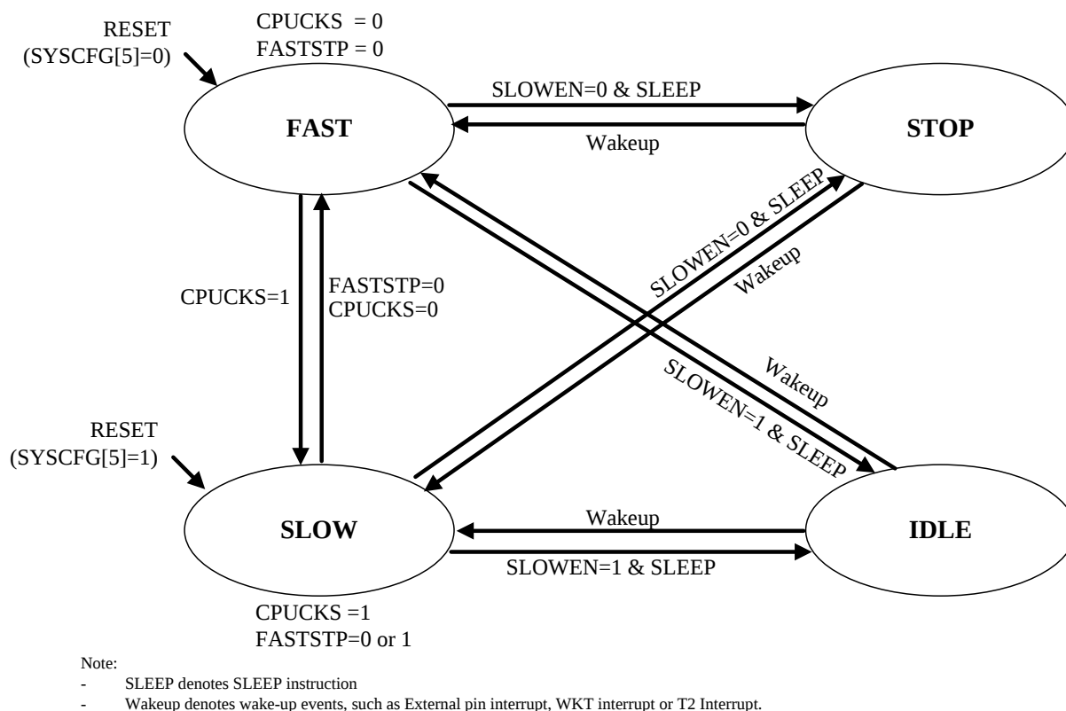
CPU Operation Block Diagram
