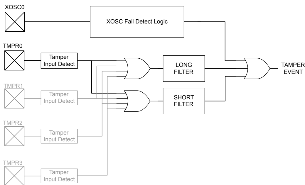
Figure 7-8. Tamper Pad with Glitch Filtering
