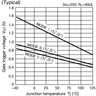
V_{GT} temperature characteristics
