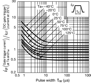
I_{GT} temperature characteristics
