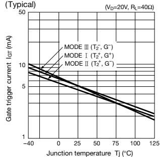
I_{GT} temperature characteristics
