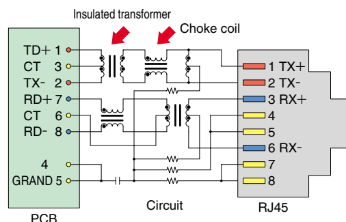
Pulse Transformer Circuit Diagram
