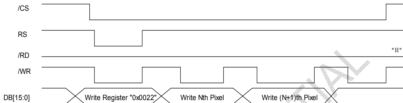
Figure 4.3.1.1 16 bit Write data
