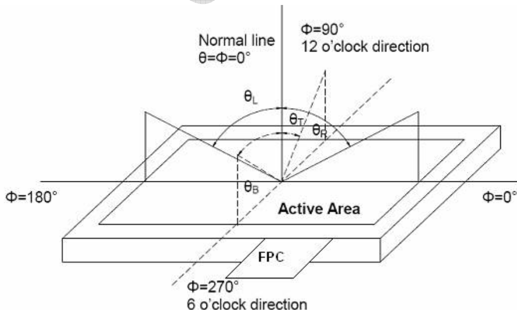
Fig.6. 1 Definition of viewing angle
