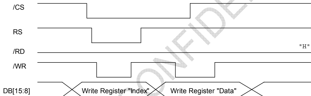
Figure 4.2.2 16-bit System Bus Interface Timing (Register Write Timing)
