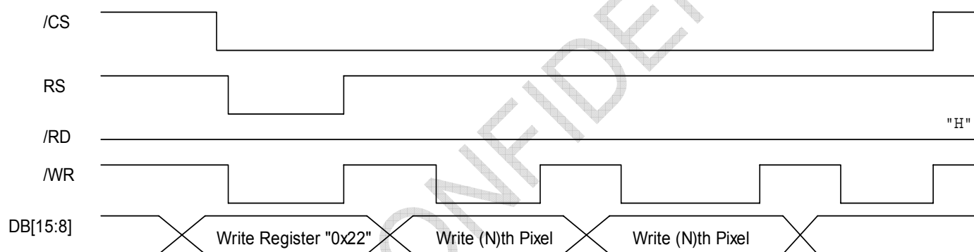
Figure 4.3.1.2 8 bit Write data
