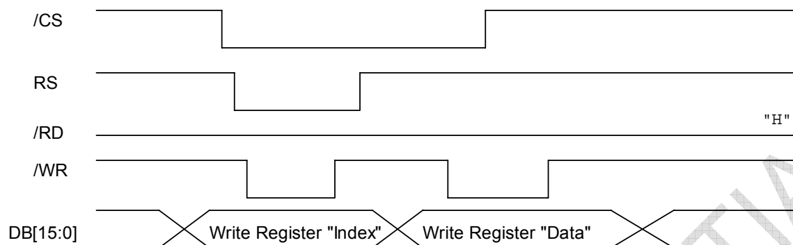
Figure 4.2.1 16-bit System Bus Interface Timing (Register Write Timing)
