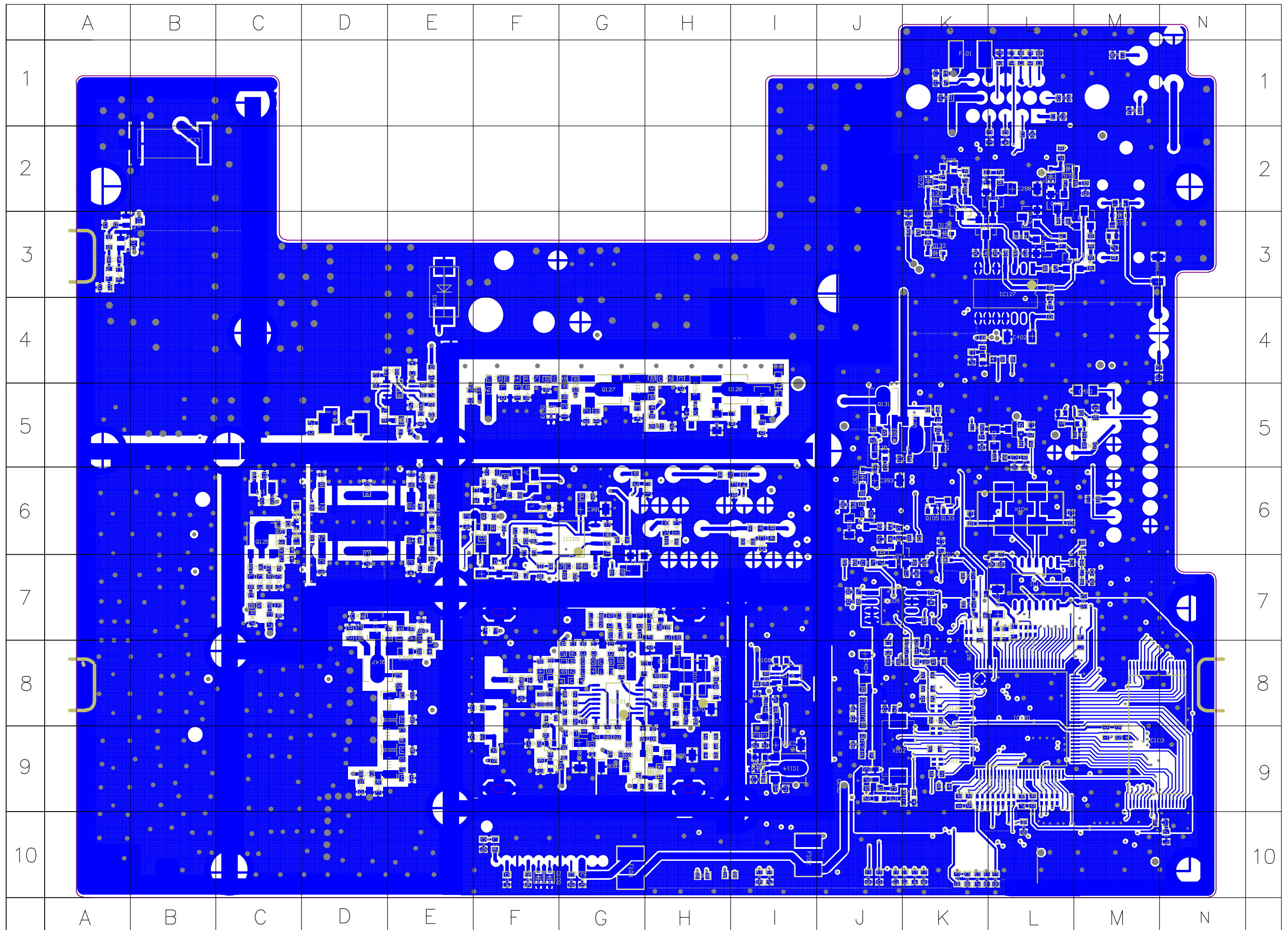
TM-800 Tx-Rx Unit (Bottom Layer)
