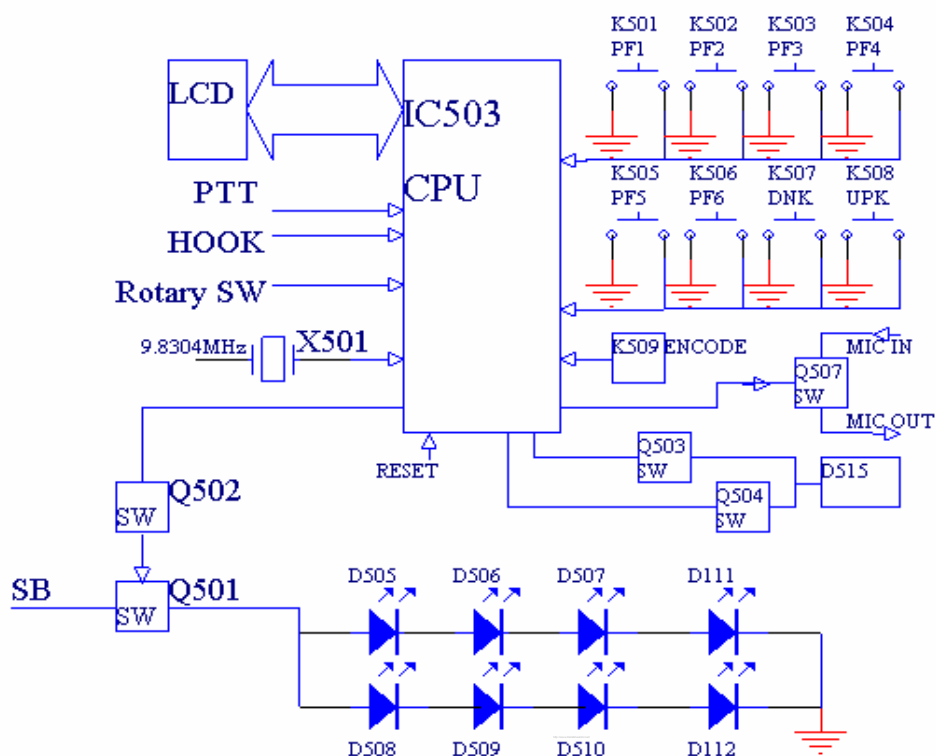
Figure 6 Display Circuit
