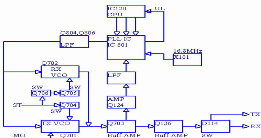
Figure 3 PLL Circuit
