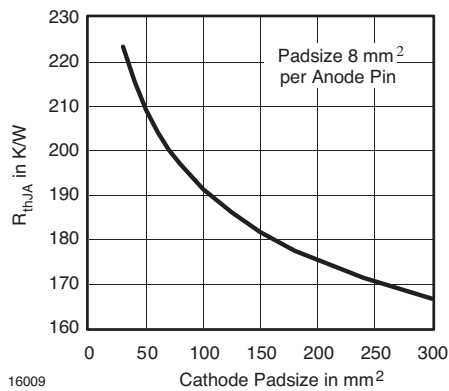
Figure 6. Thermal Resistance Junction Ambient vs. Cathode Padsize
