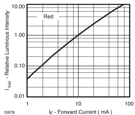
Figure 10. Relative Luminous Flux vs. Forward Current
