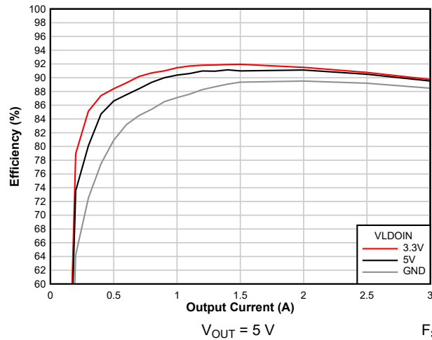
Figure 7-5. Efficiency improvements with VLDOIN ( V_{OUT} = 5\text{ V} )
