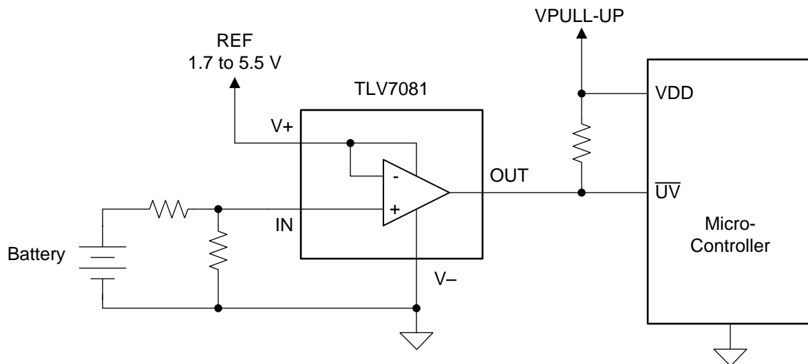
Figure 21. Under-Voltage Detection
