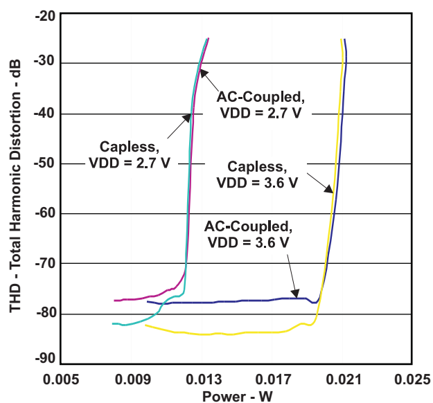
Figure 7. Headphone Power vs THD, 32 \Omega Load
