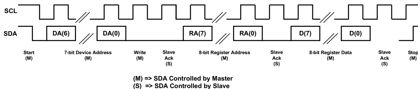
Figure 16. I2C Write
